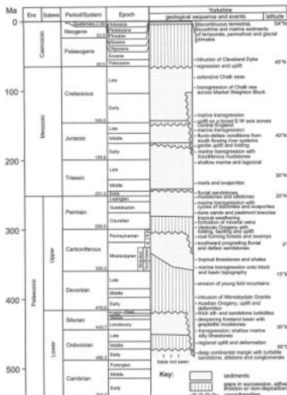
Figure 2 Geological column and sequence of events in Yorkshire. 'The terms Dinantian, Namurian (N), Westphalian (W) and Stephanian (S) no longer have formal status but are retained here for convenience.
