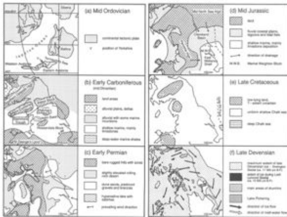
Figure 3 Palaeogeographic maps indicating: (a) the distribution of continental plates in the mid Ordovician (based on Scotese & McKerrow 1990) and (b-f) the distribution of land and major sedimentary environments at various times in Yorkshire and surrounding areas (based on Cope, et al. 1992 and other sources).
