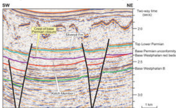
Figure 17 Seismic profile across an untested base Permian closure.
