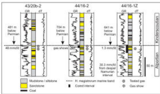
Figure 13 Examples of well sections through Alportian gas reservoirs in blocks 43/20 and 44/16.
