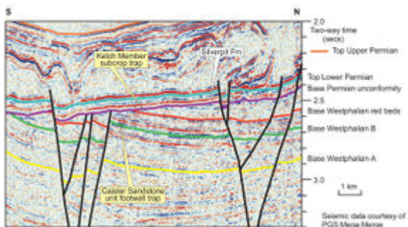
Figure 18 Seismic profile illustrating two types of intra-Carboniferous trap in block 44/19 (Department of Trade and Industry 2002: Prospect 44/19C).
