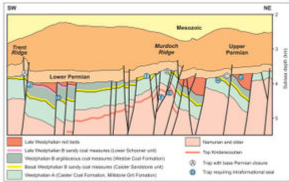
Figure 16 Geoseismic section illustrating examples of Carboniferous trap styles.
