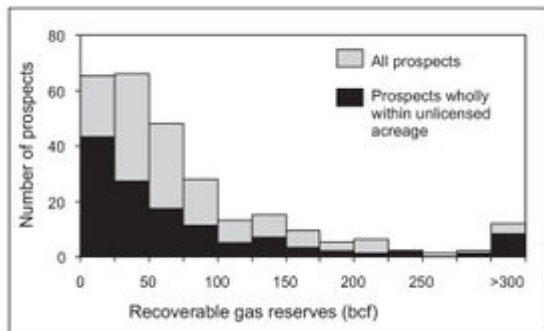
Figure 20 Histogram of P50 recoverable reserves for 279 prospects mapped by BGS in the Carboniferous fairway.
