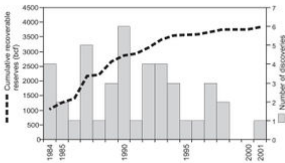
Figure 4 Graph of cumulative recoverable gas reserves, and histogram of annual gas discoveries in the Carboniferous fairway.
