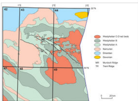
Figure 6 Pre-Permian subcrop map of the
