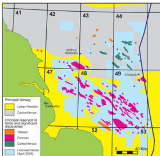
Figure 1 Southern North Sea play fairways.
