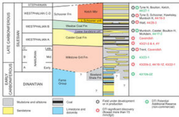
Figure 2 Simplified stratigraphical column through the Carboniferous of the southern North Sea showing stratigraphical position of selected gas discoveries.
