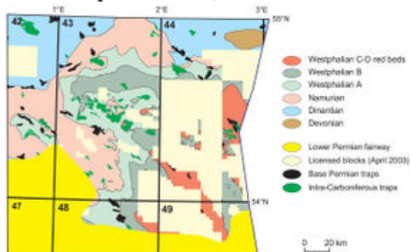
Figure 19 Distribution of undrilled traps in unlicensed acreage, mapped by BGS in the southeast of the Carboniferous fairway.
