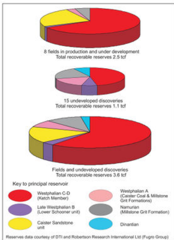
Figure 5 Proportions of recoverable gas reserves in each of the principal reservoir units of the Carboniferous fairway.
