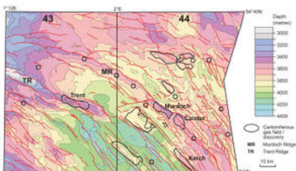
Figure 15 Depth in metres to the base
