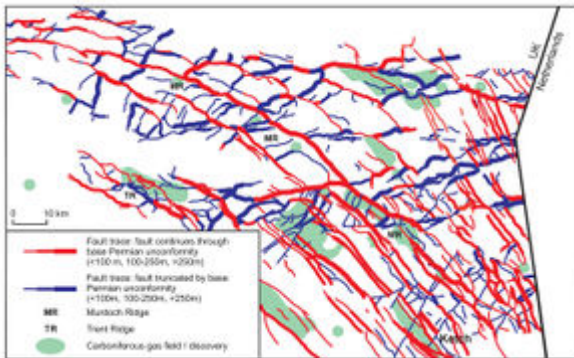
Figure 7 Intra-Carboniferous fault pattern in the southeast of the Carboniferous fairway.
