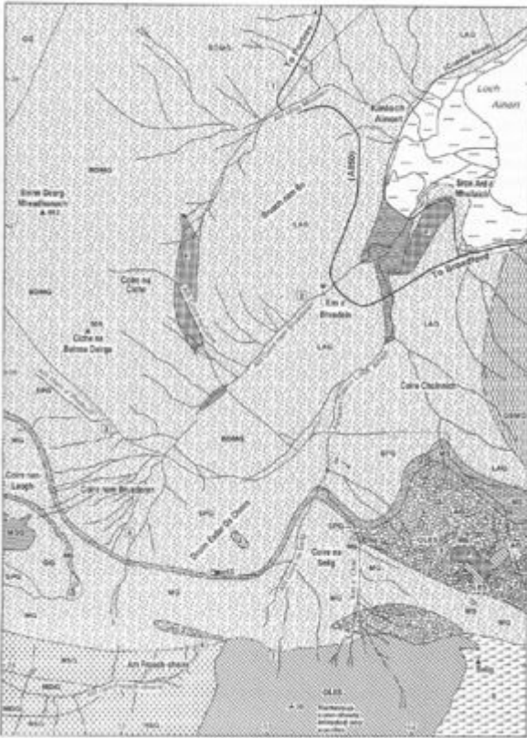
Figure 26 Excursion 12 Gleann Torra-mhichaig-Coire nam Bruadaran-Belig, location map Key to symbols
